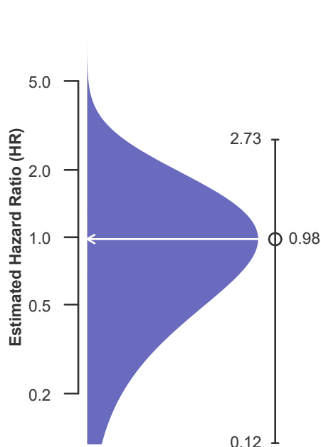
Figure C21PTA. Adult (18+) 3-year patient death HR estimate (deceased donor grafts): (PTA)
